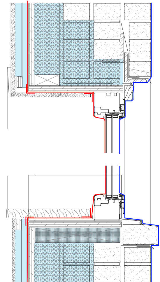
WINDOW DETAIL SECTION
