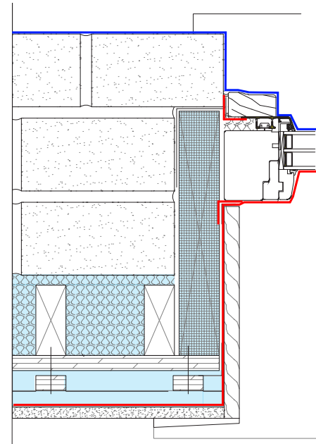
WINDOW DETAIL PLAN
