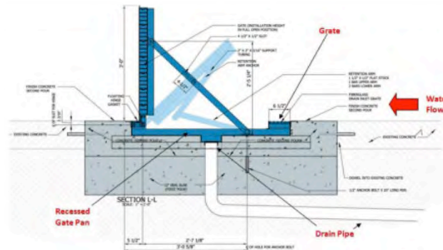
STRUCTURAL REINFORCEMENT - Passive and Manual
