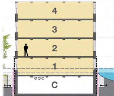
DRY FLOOD PROOFING - Passive
