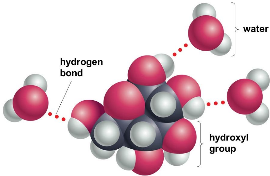
Figure 3-4 Sugar dissolving in water
